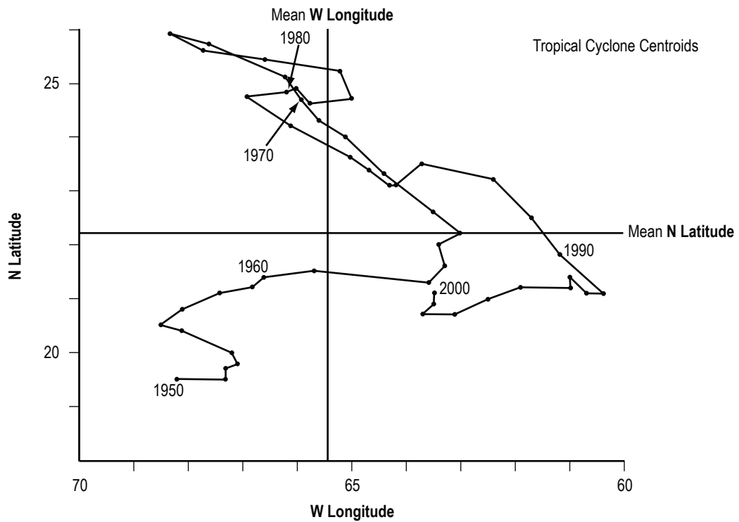
Figure 3. The time-ticked variation of the GL centroids, latitude, and longitude for tropical cyclones (lower panel) and hurricanes (upper panel). The thin vertical and horizontal lines are the long-term means.
