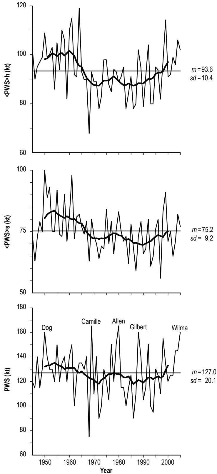
Figure 4. The yearly variation of PWS (lower panel), \langle PWS \rangle_s (middle panel), and \langle PWS \rangle_h (upper panel). The thin jagged lines are the yearly values, the thick smooth lines are the 10-yr moving averages, and the thin horizontal lines are the long-term means.
